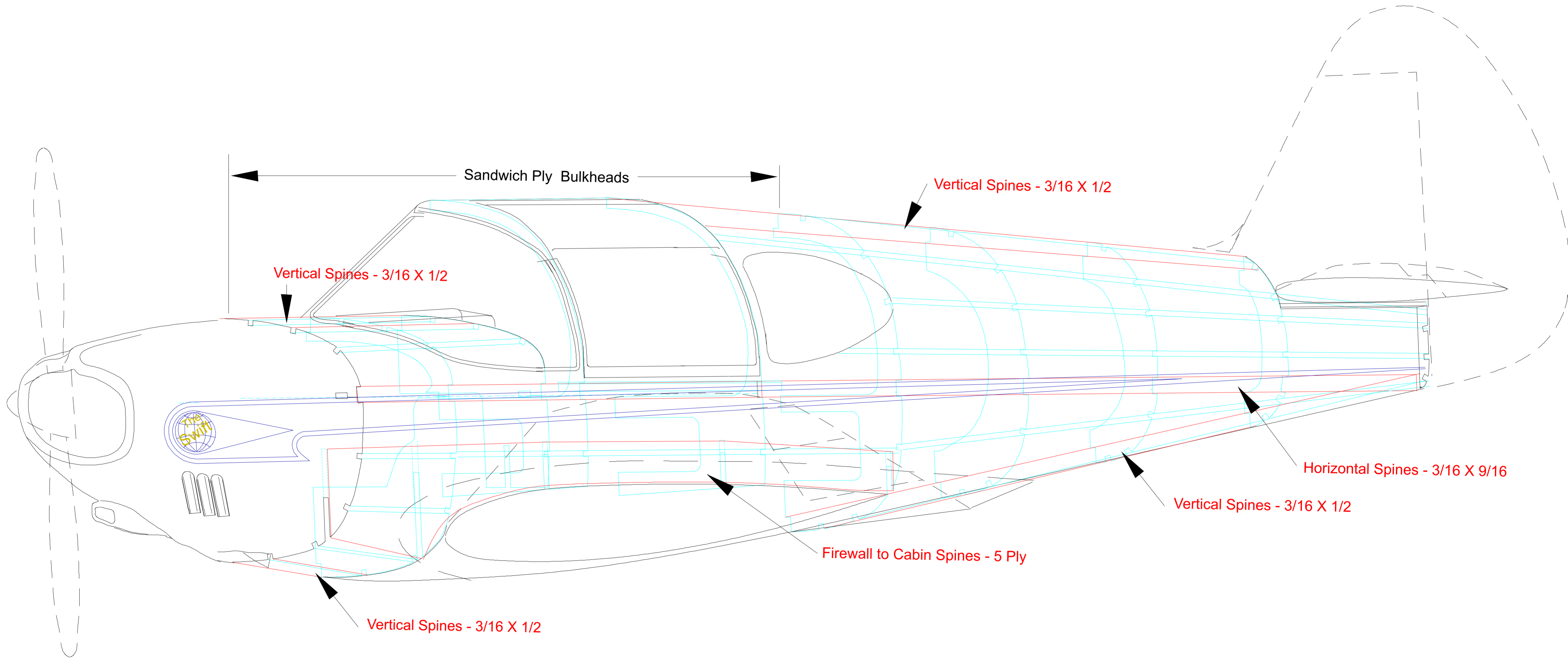
Swift Fuselage Construction
